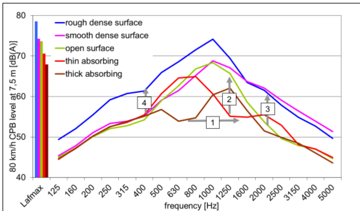
Figure 2.1: Spectral distribution of the different aging processes: (1) filling up of the lower layer, (2) further filling, (3) clogging of top-layer and (4) stone loss. Spectra are
