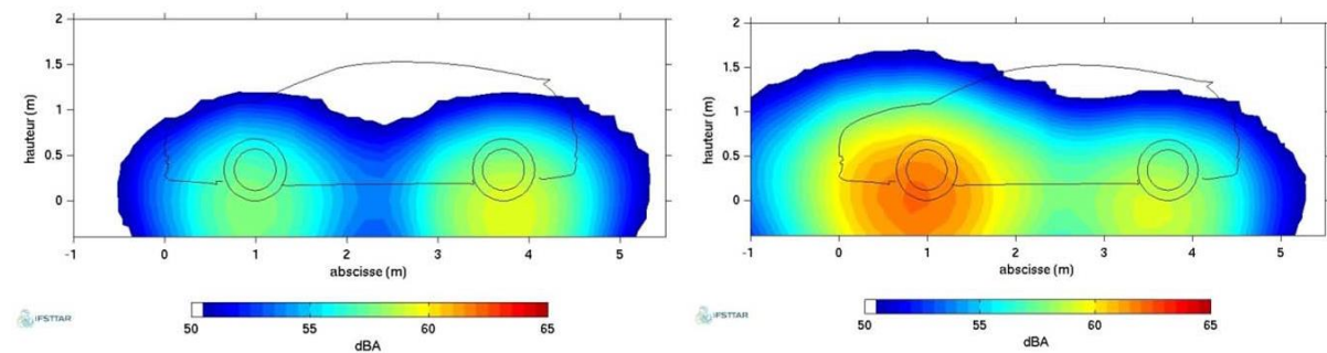
Figure 2.5: Noise maps of HEVs in electrical and hybrid mode [23]
